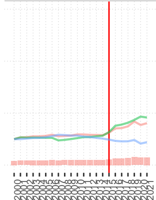
Cerebrovascular disease_AHRQ
